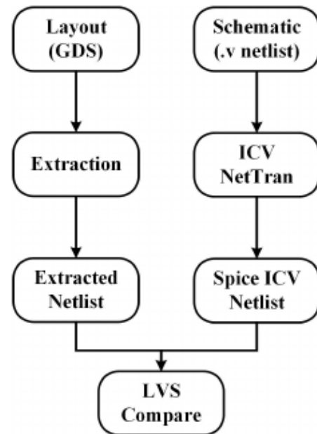
FIGURE 2.10 LVS Flow.
