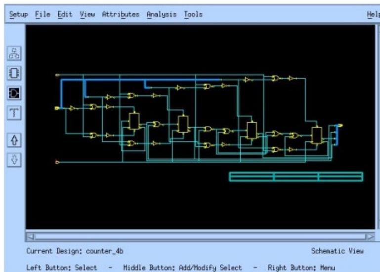
FIGURE 2.6 The Schematic View of ASIC Synthesis.
